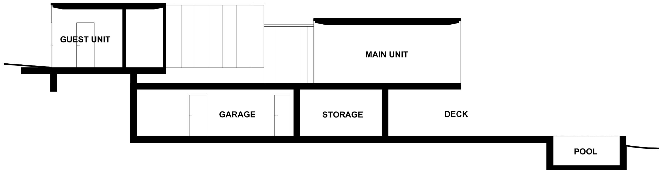
SECTION B-B
